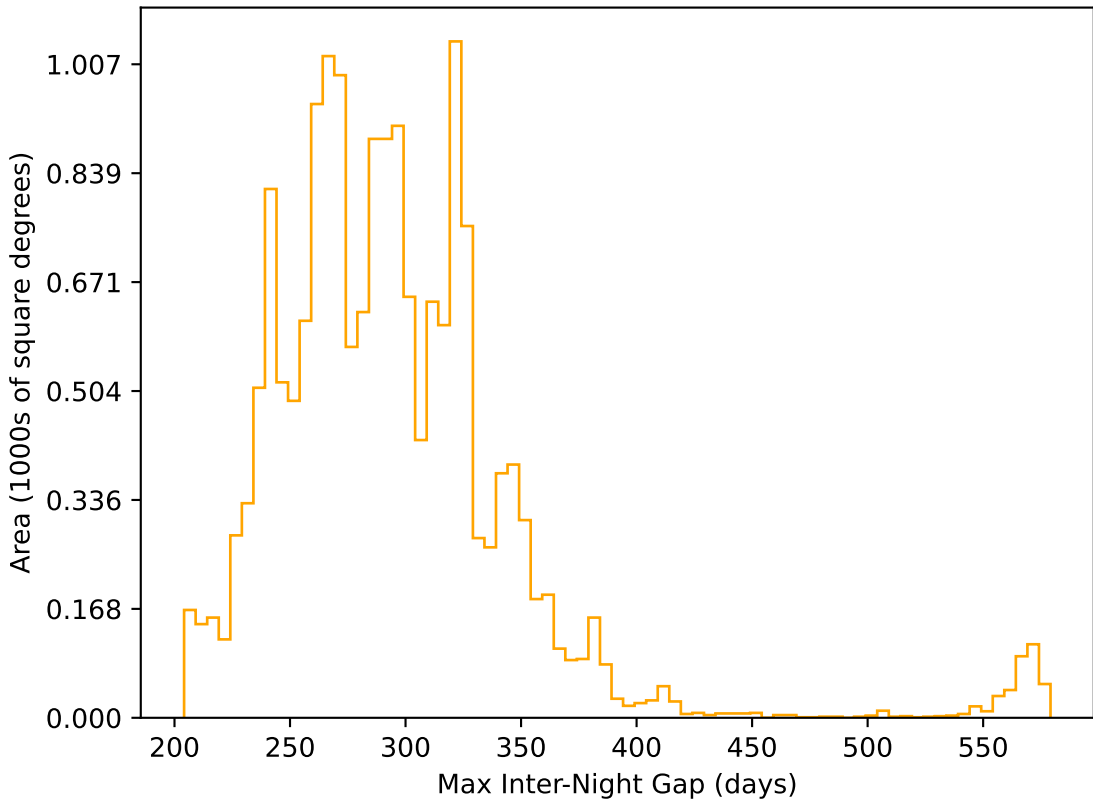
weather_cloudso31v3.4_10yrs WFD r band: Max Inter-Night Gap
