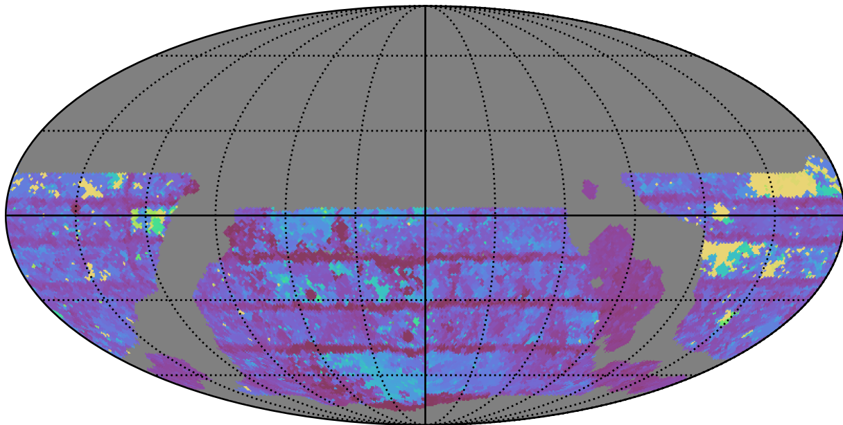
weather_cloudso31v3.4_10yrs WFD i band: Max Inter-Night Gap
