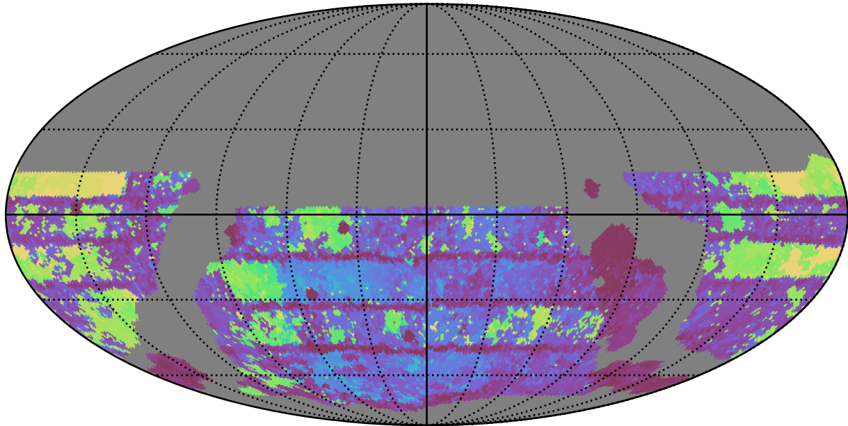
weather_cloudso31v3.4_10yrs WFD g band: Max Inter-Night Gap
