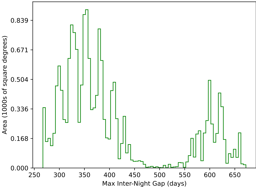
weather_cloudso31v3.4_10yrs WFD g band: Max Inter-Night Gap
