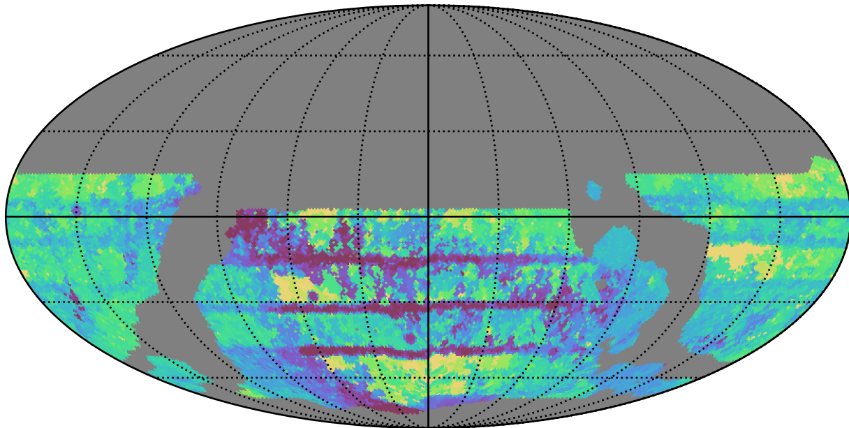
weather_cloudso31v3.4_10yrs WFD all bands: Max Inter-Night Gap
