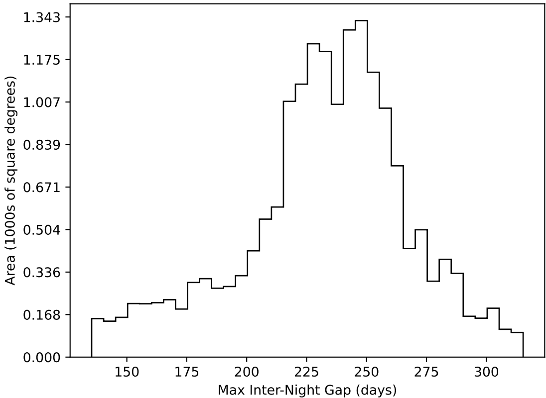
weather_cloudso31v3.4_10yrs WFD all bands: Max Inter-Night Gap
