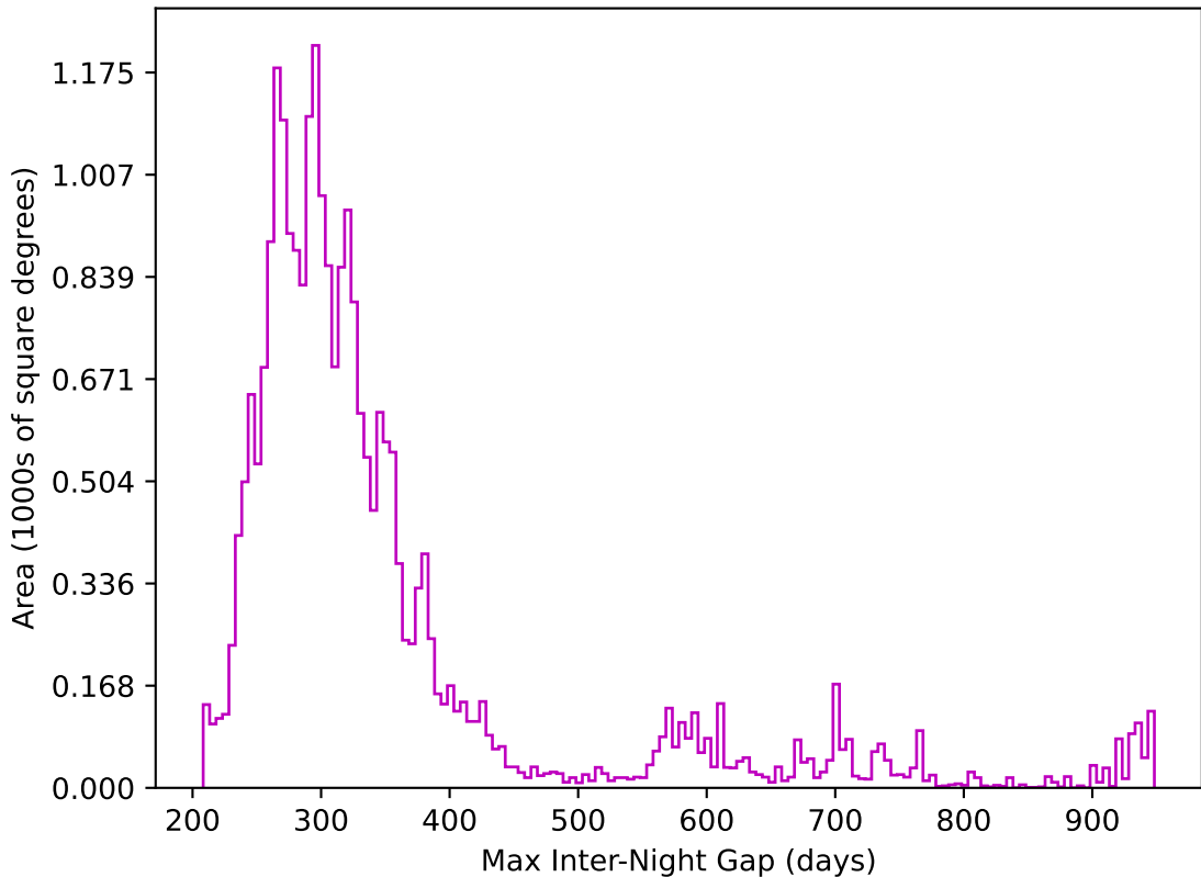
weather_cloudso31v3.4_10yrs All sky z band: Max Inter-Night Gap
