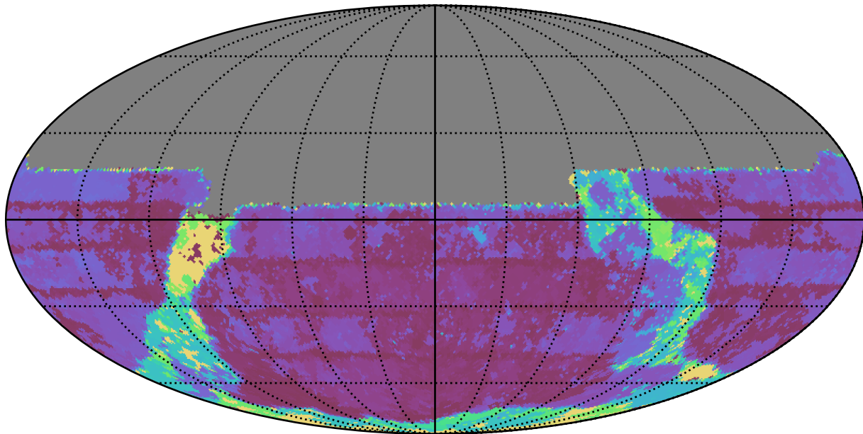
weather_cloudso31v3.4_10yrs All sky u band: Max Inter-Night Gap
