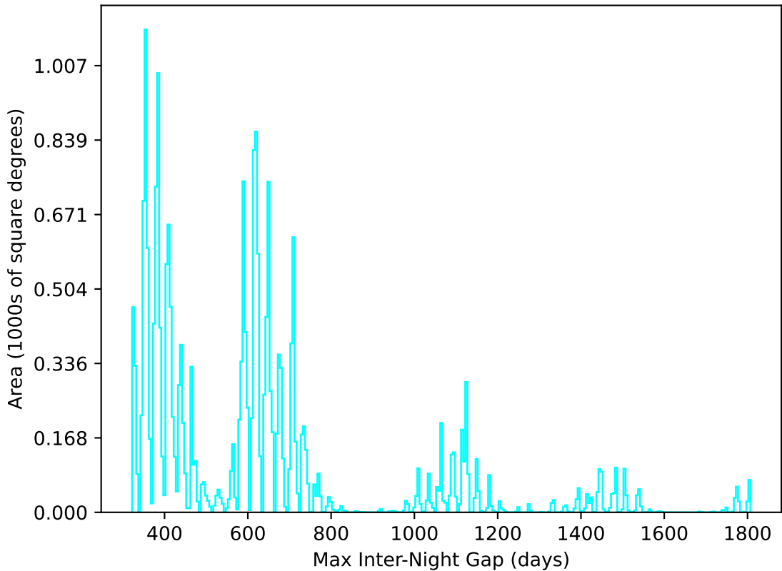
weather_cloudso31v3.4_10yrs All sky u band: Max Inter-Night Gap
