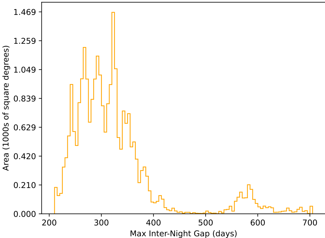
weather_cloudso31v3.4_10yrs All sky r band: Max Inter-Night Gap
