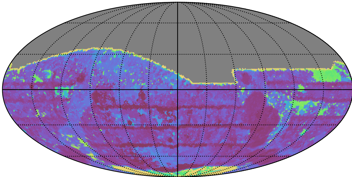
weather_cloudso31v3.4_10yrs All sky i band: Max Inter-Night Gap
