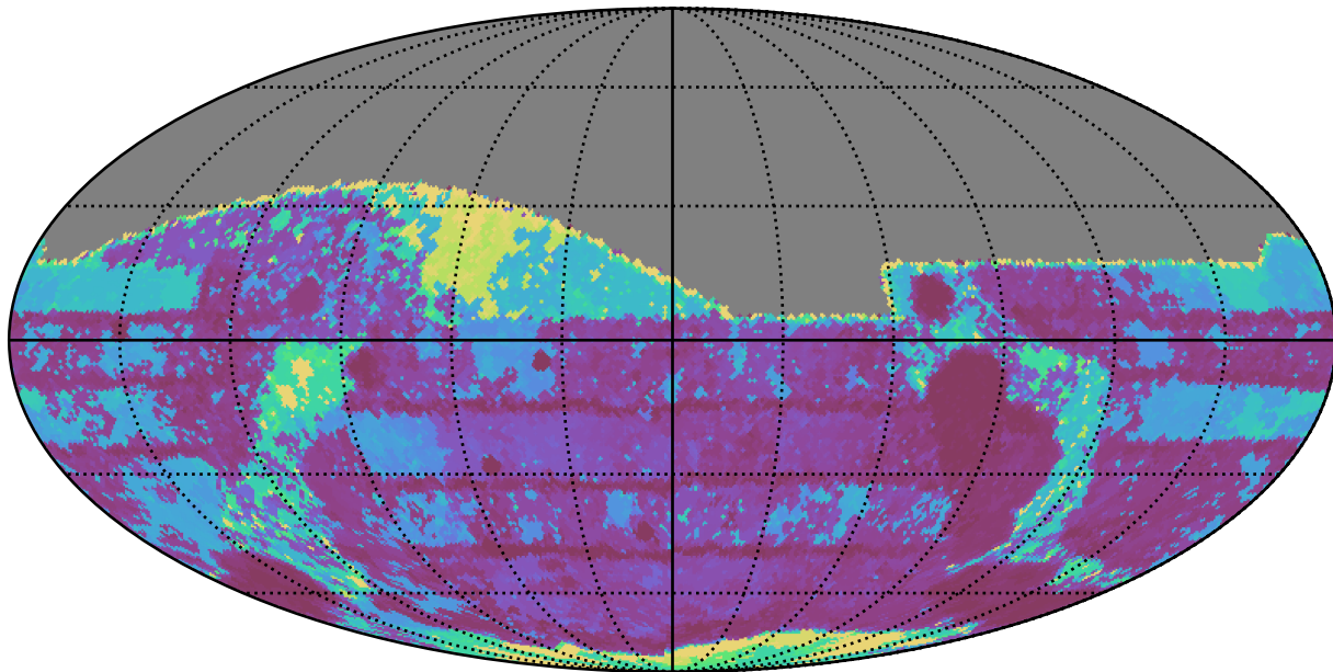
weather_cloudso31v3.4_10yrs All sky g band: Max Inter-Night Gap
