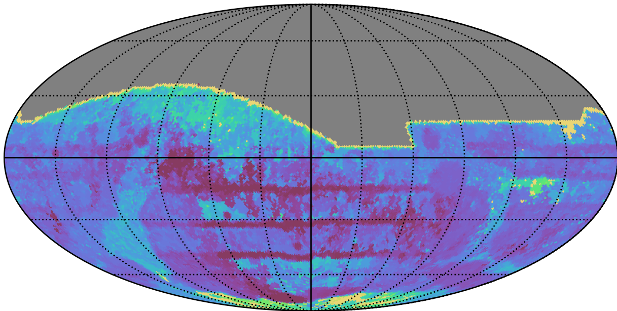
weather_cloudso31v3.4_10yrs All sky all bands: Max Inter-Night Gap
