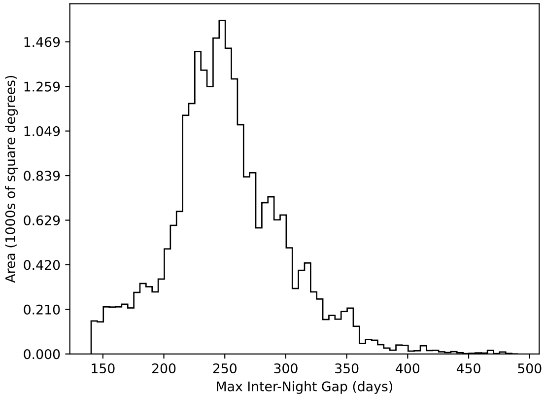
weather_cloudso31v3.4_10yrs All sky all bands: Max Inter-Night Gap
