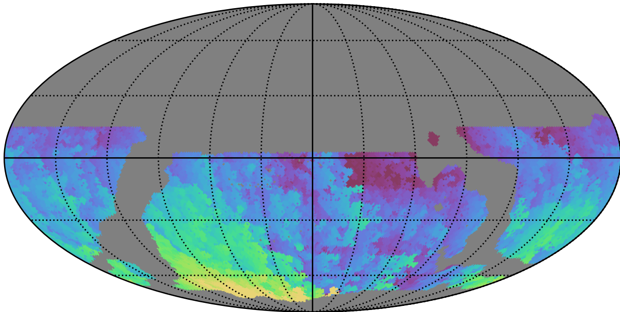
weather_cloudso31v3.4_10yrs WFD u band: Max HA
