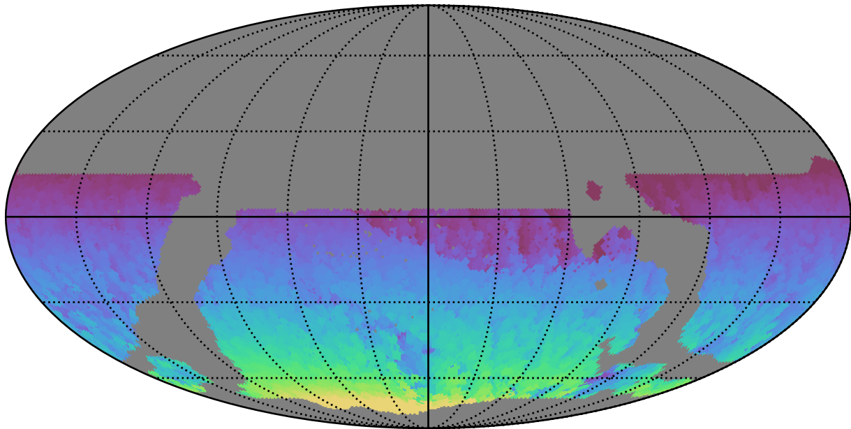
weather_cloudso31v3.4_10yrs WFD all bands: Max HA
