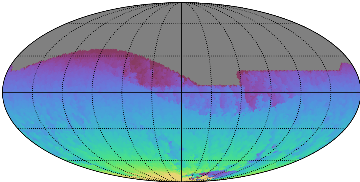
weather_cloudso31v3.4_10yrs All sky all bands: Max HA
