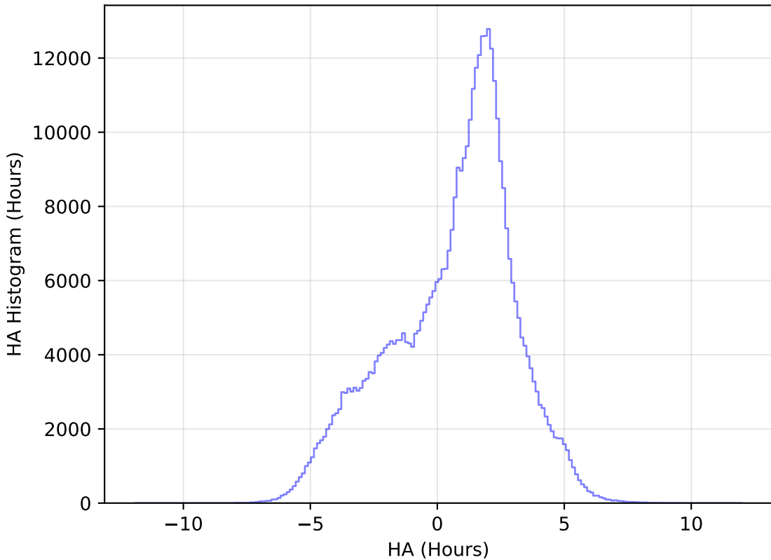
weather_cloudso31v3.4_10yrs WFD z band: HA Histogram
