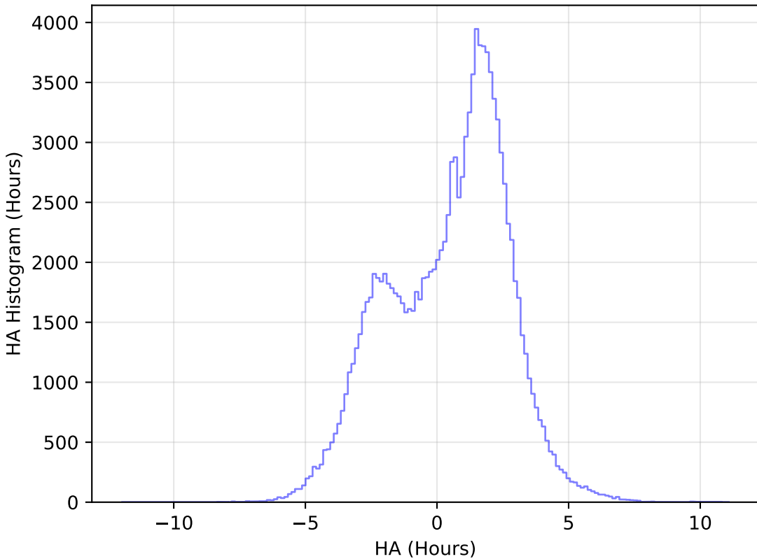
weather_cloudso31v3.4_10yrs WFD u band: HA Histogram
