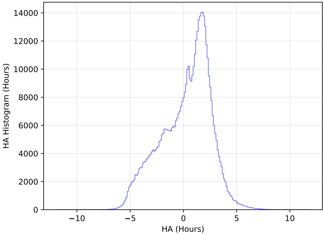
weather_cloudso31v3.4_10yrs WFD r band: HA Histogram
