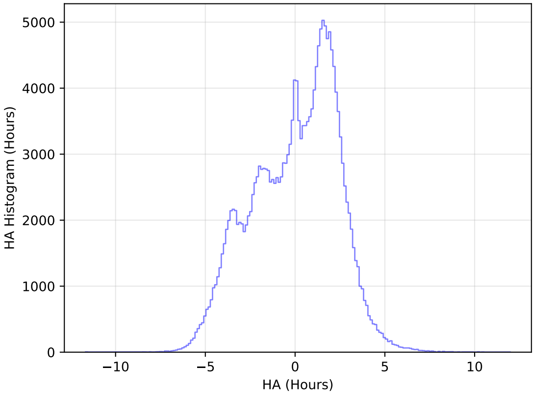
weather_cloudso31v3.4_10yrs WFD g band: HA Histogram
