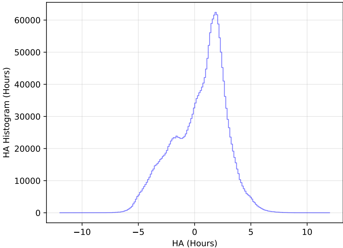
weather_cloudso31v3.4_10yrs All sky all bands: HA Histogram
