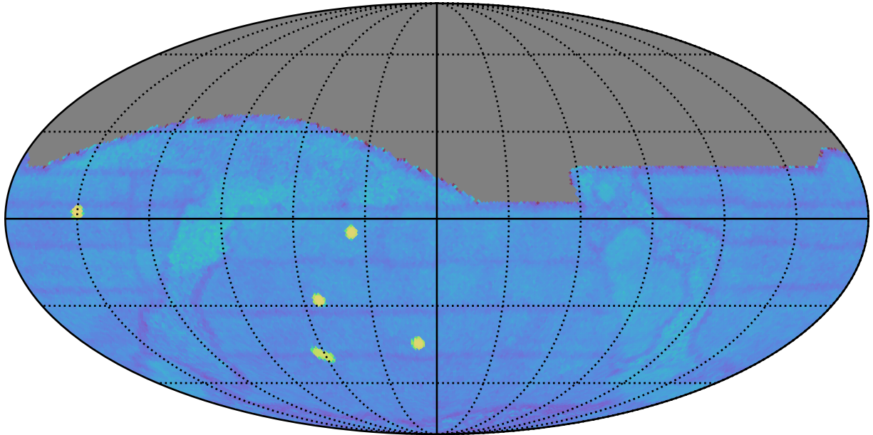
weather_cloudso31v3.4_10yrs gri All sky: Fraction of visits with a revisit < 60 min
