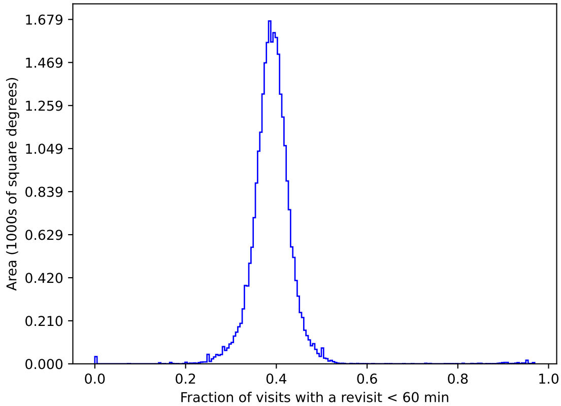
weather_cloudso31v3.4_10yrs gri All sky: Fraction of visits with a revisit < 60 min
