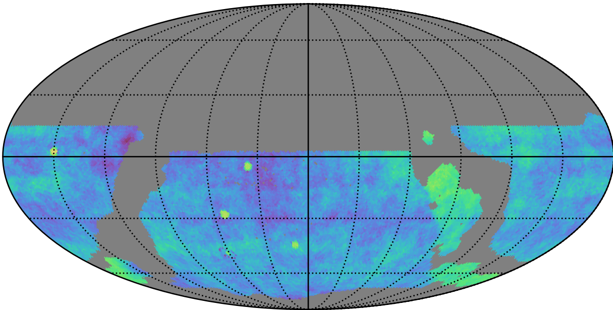
weather_cloudso31v3.4_10yrs gri WFD: Fraction of visits in pairs (20-90 min)
