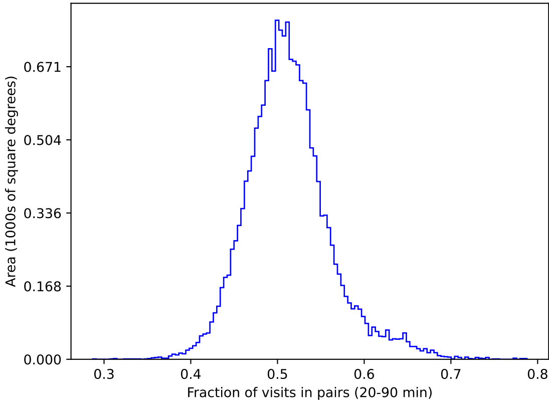
weather_cloudso31v3.4_10yrs gri WFD: Fraction of visits in pairs (20-90 min)
