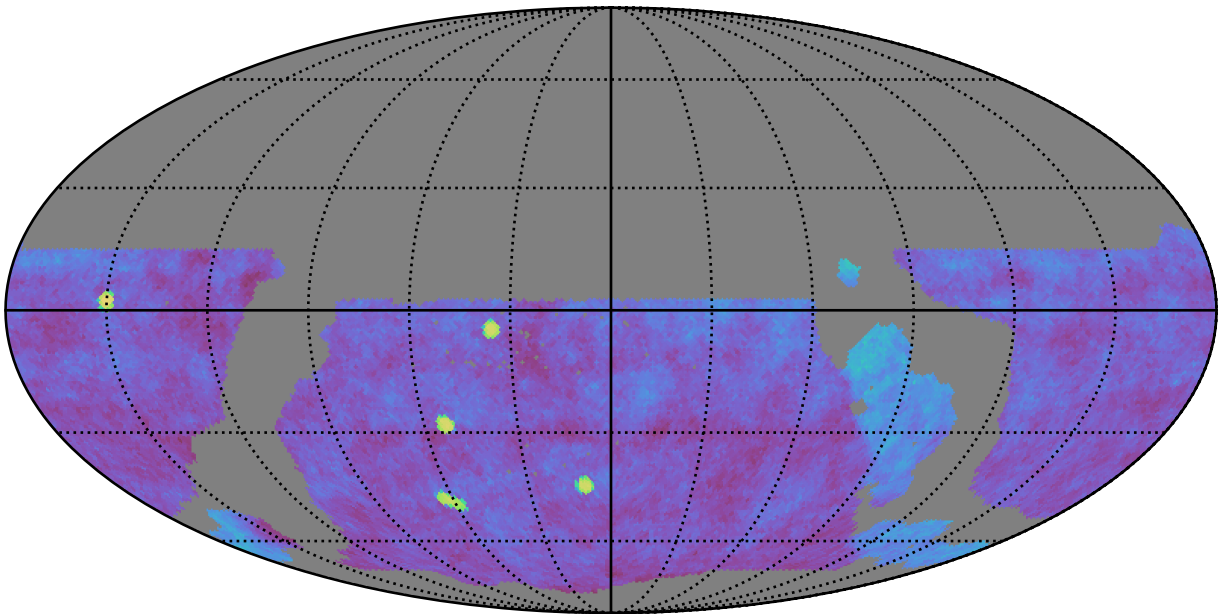
weather_cloudso31v3.4_10yrs gri WFD: Fraction of visits in pairs (10-60 min)
