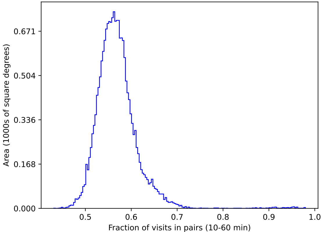
weather_cloudso31v3.4_10yrs gri WFD: Fraction of visits in pairs (10-60 min)
