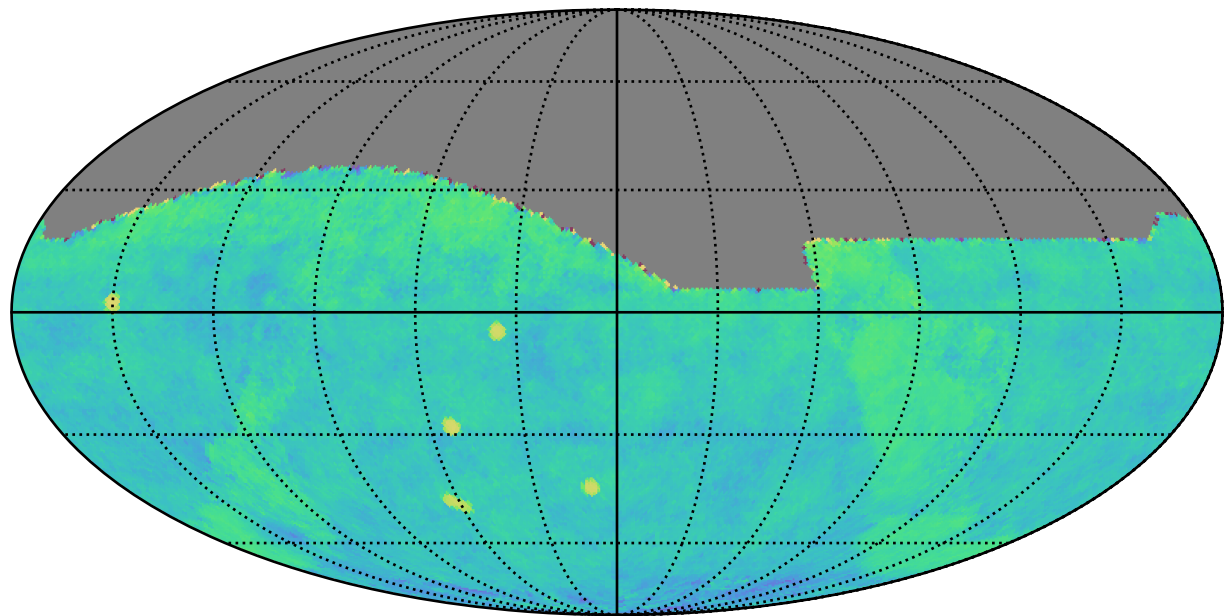
weather_cloudso31v3.4_10yrs gri All sky: Fraction of visits in pairs (10-60 min)
