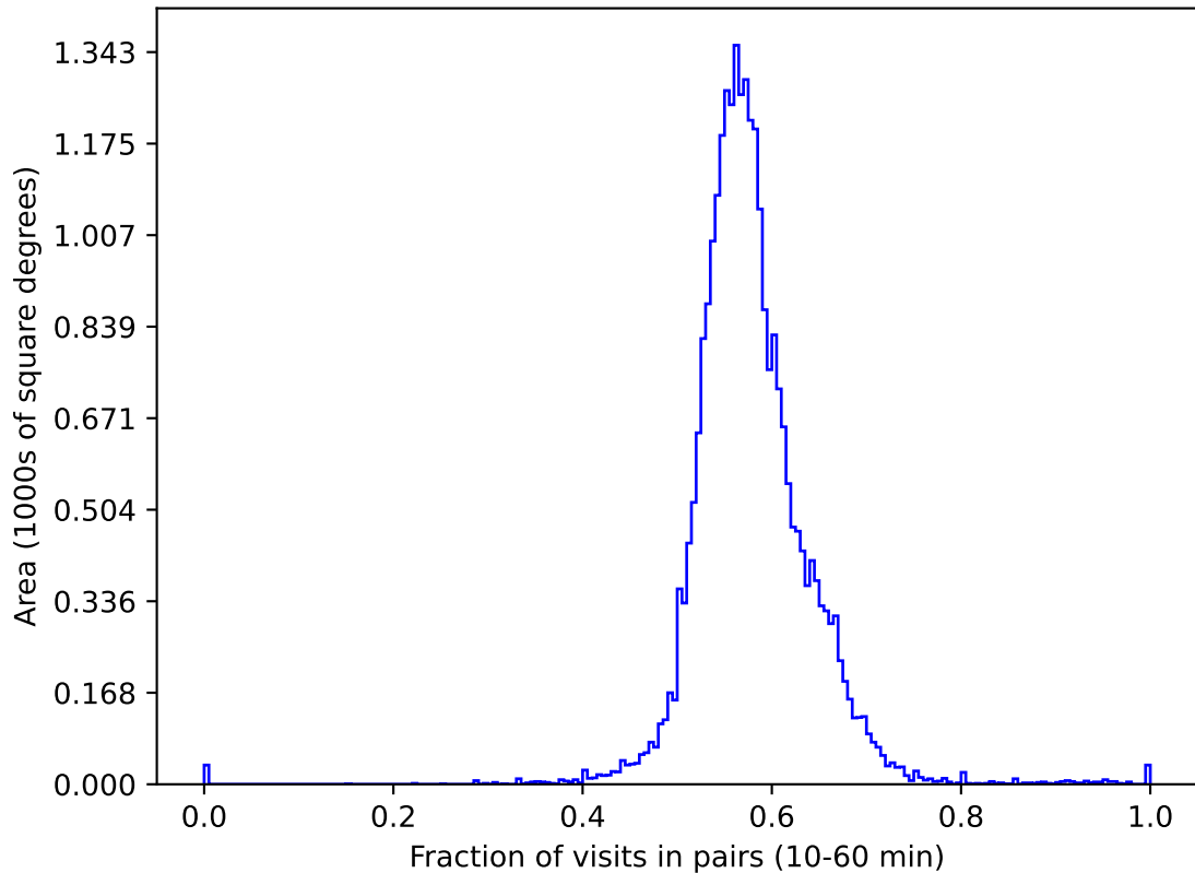
weather_cloudso31v3.4_10yrs gri All sky: Fraction of visits in pairs (10-60 min)
