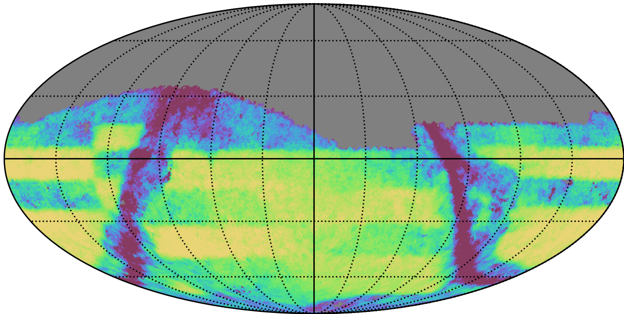
weather_cloudso31v3.4_10yrs Yr 3-4 z band: Exgal_CoaddM5
