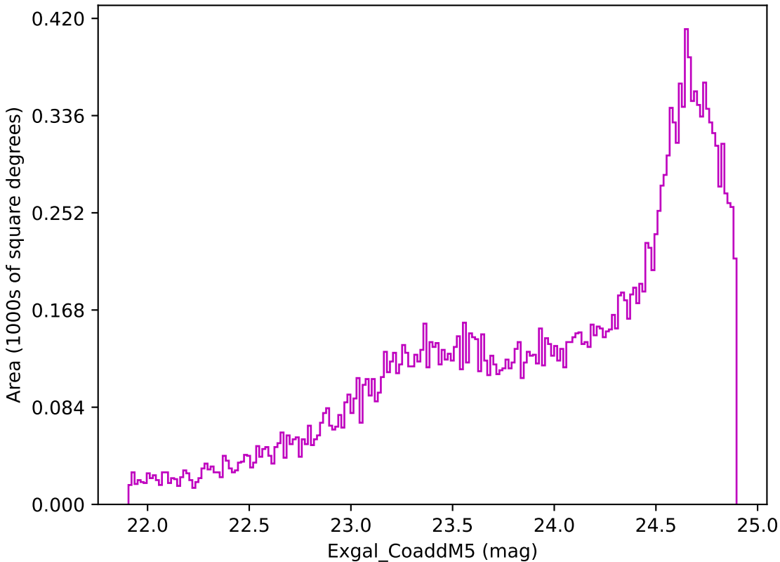
weather_cloudso31v3.4_10yrs Yr 3-4 z band: Exgal_CoaddM5
