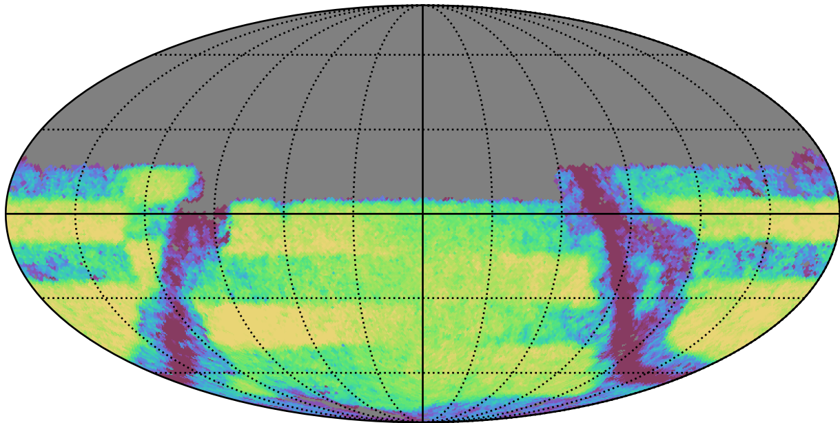
weather_cloudso31v3.4_10yrs Yr 3-4 y band: Exgal_CoaddM5
