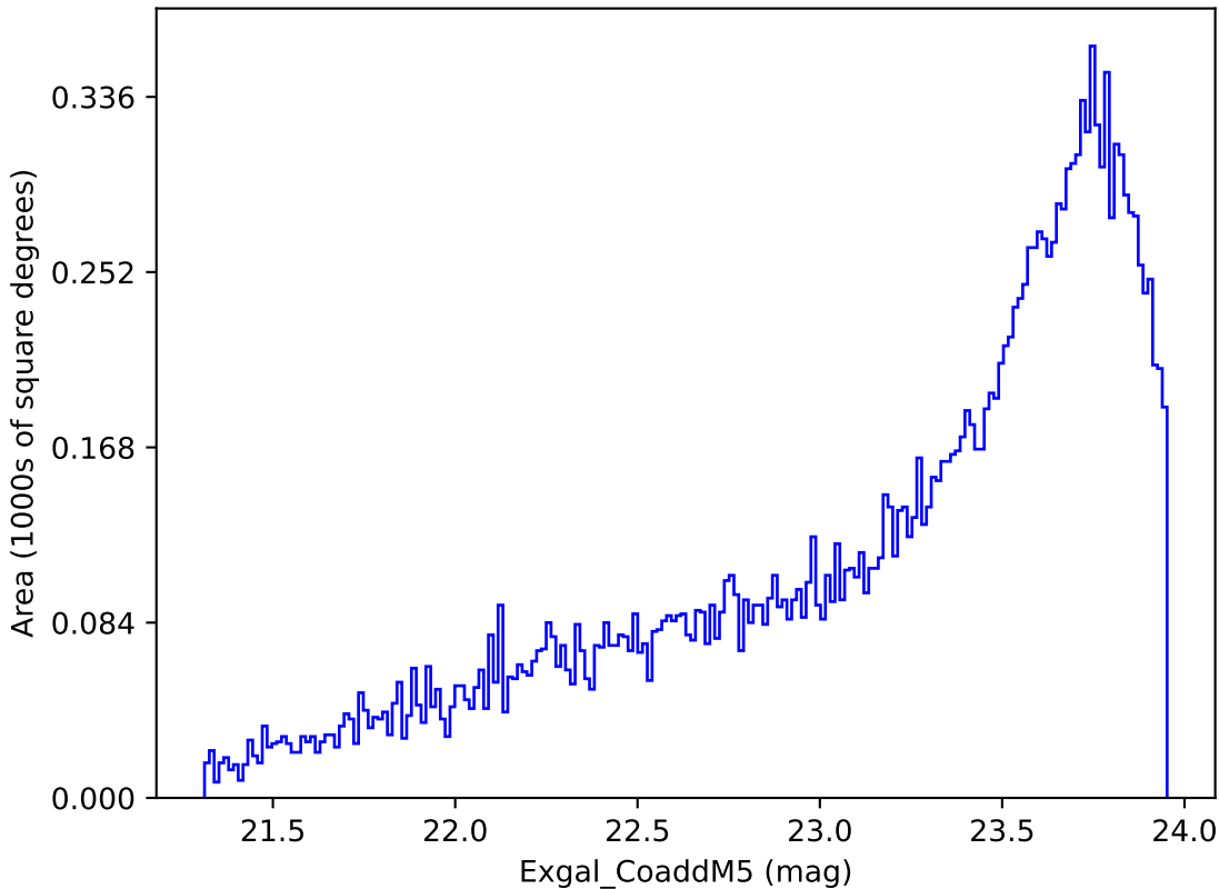
weather_cloudso31v3.4_10yrs Yr 3-4 y band: Exgal_CoaddM5
