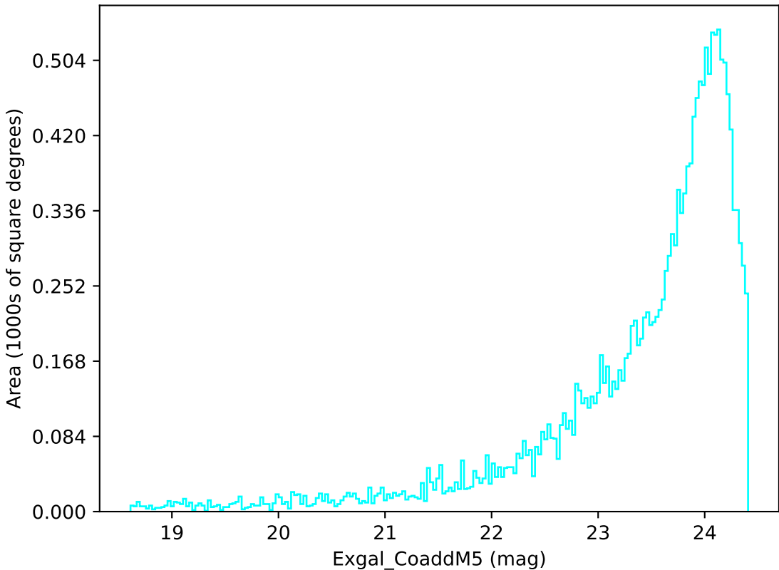
weather_cloudso31v3.4_10yrs Yr 3-4 u band: Exgal_CoaddM5
