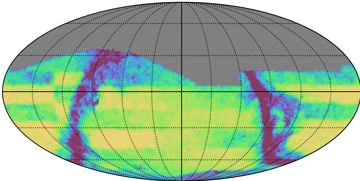
weather_cloudso31v3.4_10yrs Yr 3-4 r band: Exgal_CoaddM5
