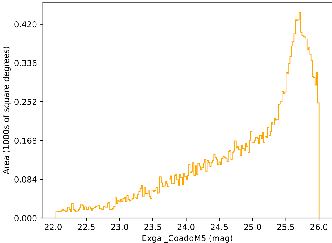
weather_cloudso31v3.4_10yrs Yr 3-4 r band: Exgal_CoaddM5
