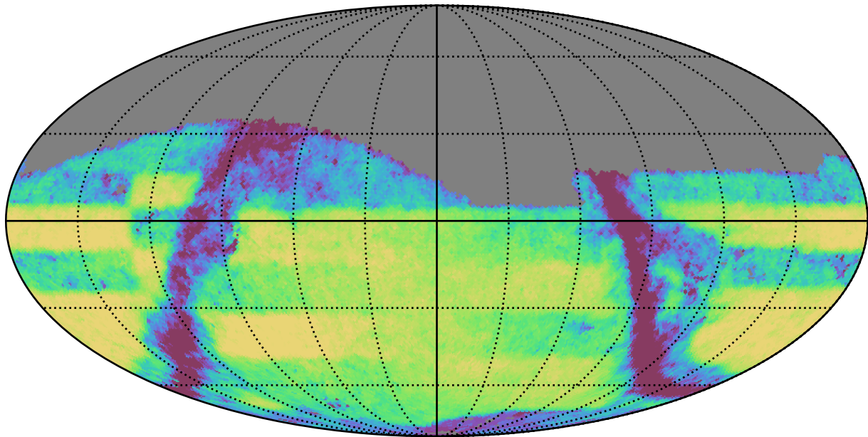
weather_cloudso31v3.4_10yrs Yr 3-4 i band: Exgal_CoaddM5
