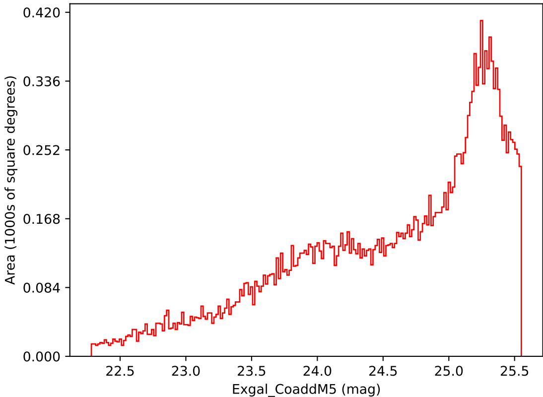
weather_cloudso31v3.4_10yrs Yr 3-4 i band: Exgal_CoaddM5
