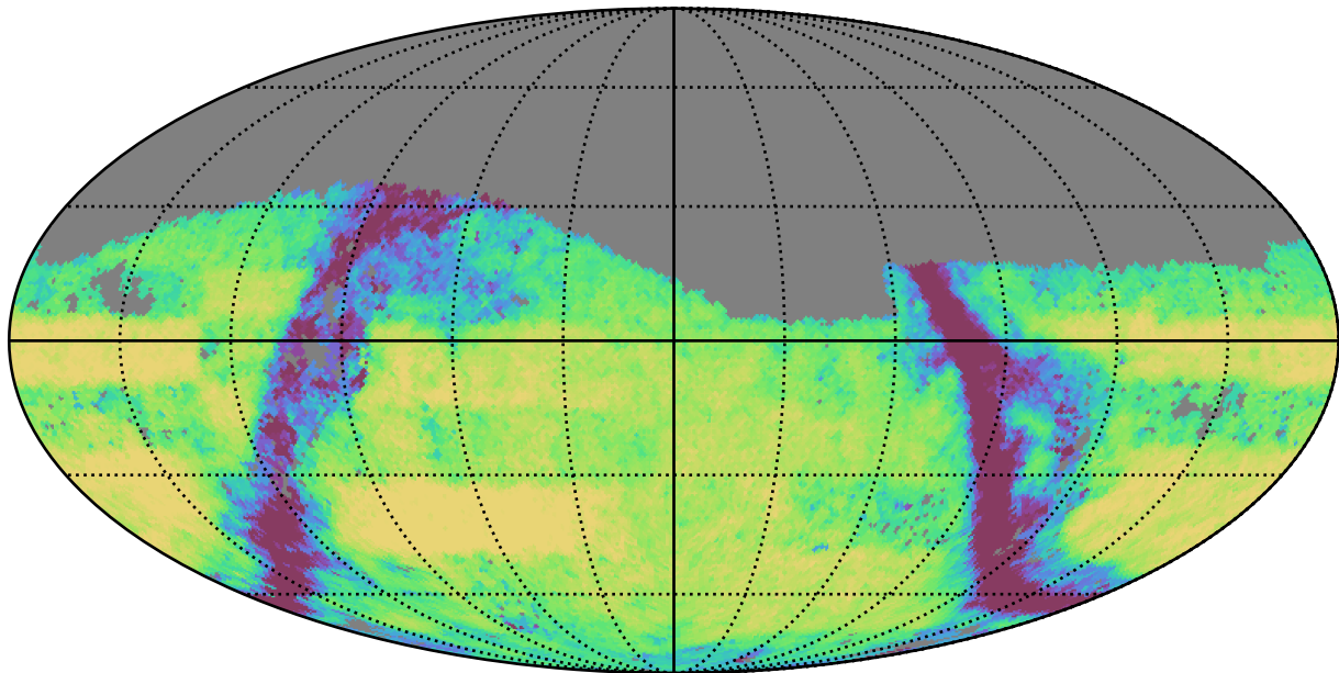
weather_cloudso31v3.4_10yrs Yr 3-4 g band: Exgal_CoaddM5
