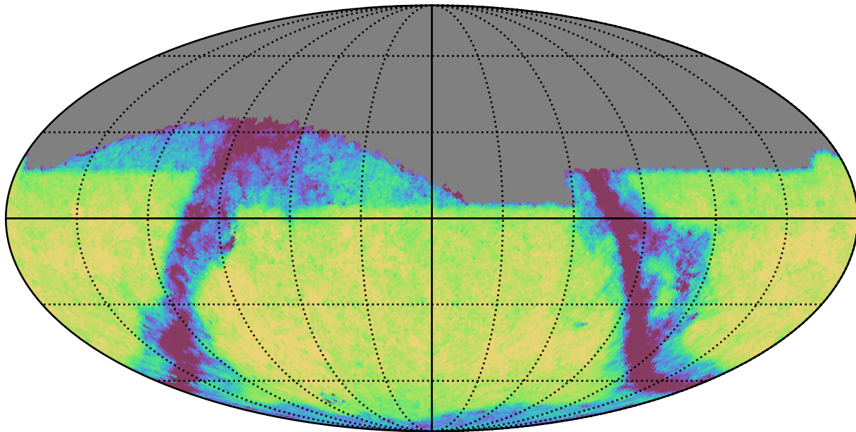
weather_cloudso31v3.4_10yrs Yr 1 z band: Exgal_CoaddM5
