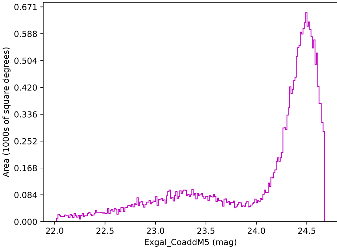
weather_cloudso31v3.4_10yrs Yr 1 z band: Exgal_CoaddM5
