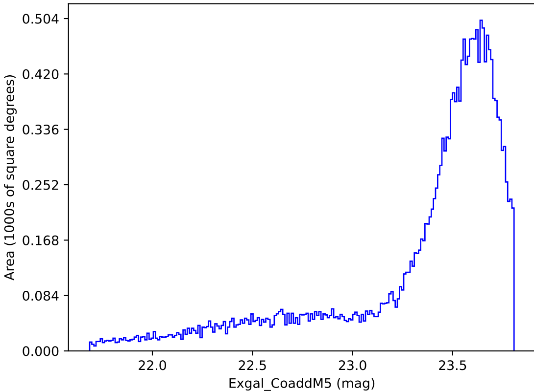
weather_cloudso31v3.4_10yrs Yr 1 y band: Exgal_CoaddM5
