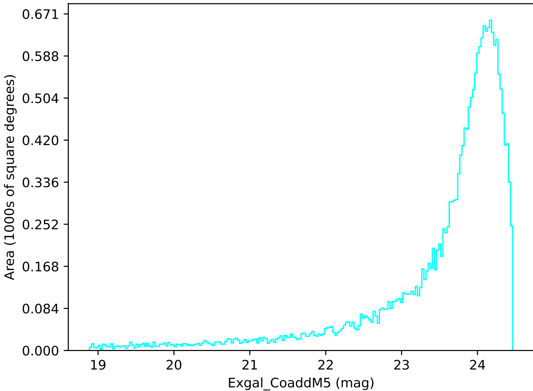
weather_cloudso31v3.4_10yrs Yr 1 u band: Exgal_CoaddM5
