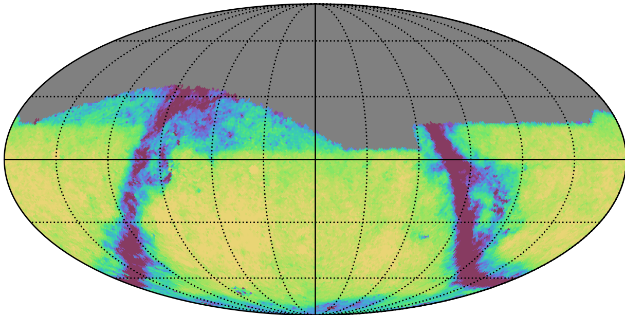
weather_cloudso31v3.4_10yrs Yr 1 r band: Exgal_CoaddM5
