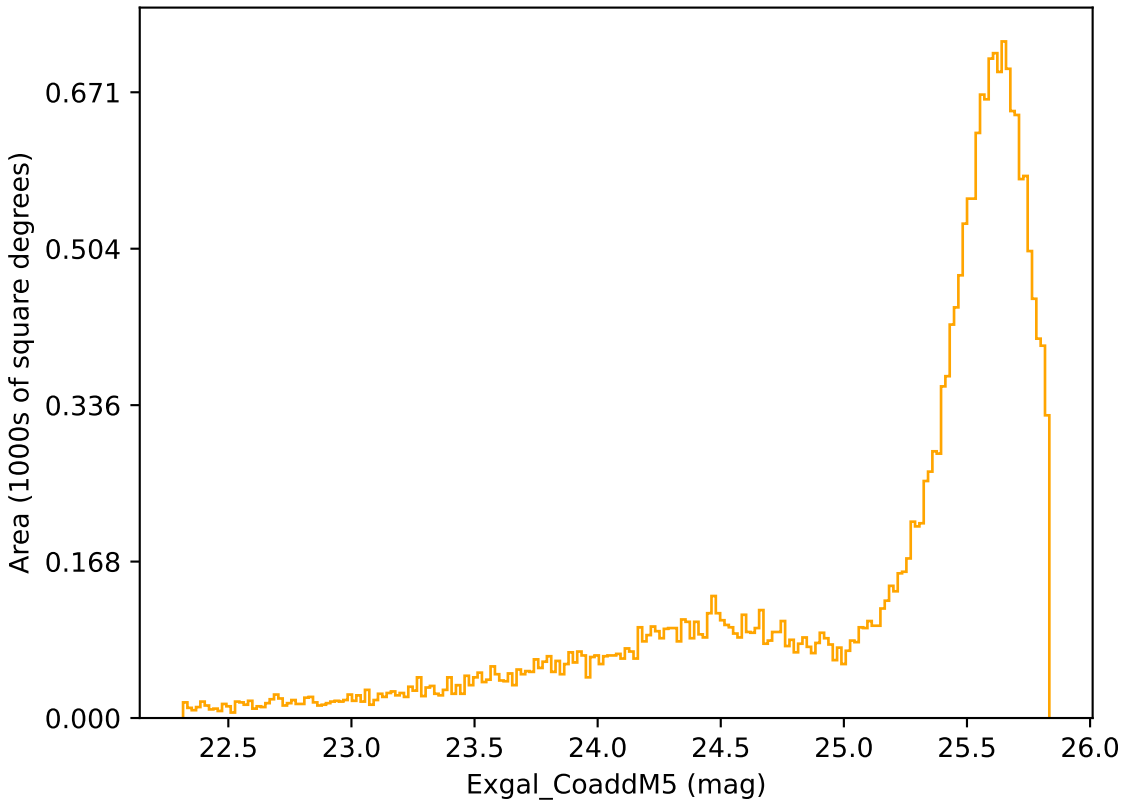
weather_cloudso31v3.4_10yrs Yr 1 r band: Exgal_CoaddM5
