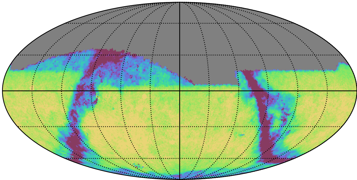
weather_cloudso31v3.4_10yrs Yr 1 i band: Exgal_CoaddM5
