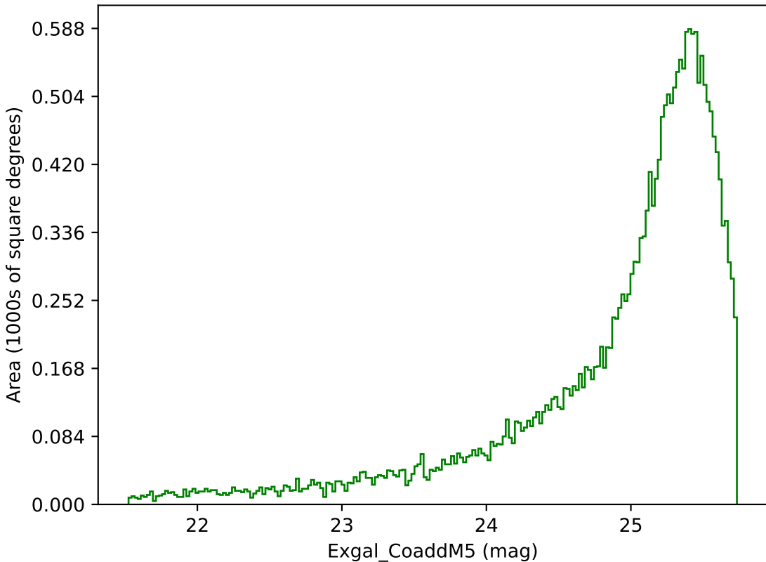
weather_cloudso31v3.4_10yrs Yr 1 g band: Exgal_CoaddM5
