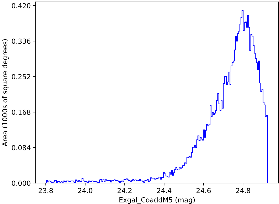
weather_cloudso31v3.4_10yrs WFD y band: Exgal_CoaddM5
