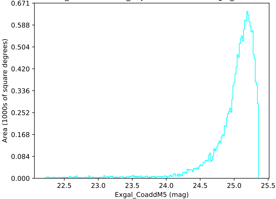
weather_cloudso31v3.4_10yrs WFD u band: Exgal_CoaddM5
